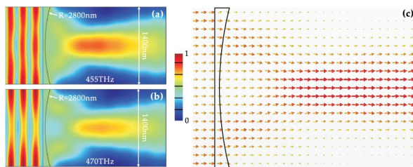
Fig. 3. (Color online) The electromagnetic waves can be focused by a two dimensional concave lens made from the ENZ meta-atom stacks at (a) 455 THz and (b) 470 THz, where the magnetic field intensity distribution is displayed. (c) The energy flow with respect to the result of (a) clearly indicates the focusing of the electromagnetic energy. Because of the large quantity of the ENZ stacks within the concave lens, the detailed structure of the lens is not displayed here.
