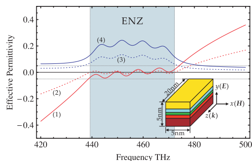
Fig. 1. (Color online) Real part and the imaginary part of the effective permittivity based on the FDTD simulation and the theoretical analysis from Eq. (1). The insert indicates the structure geometry of the broadband ENZ meta-atom stack including five layers. The theoretical effective permittivity is plotted as dashed curves, while the numerically retrieved permittivity is denoted as solid curves. In addition, the real part is shown in red color [curves (1) and (2)], and the imaginary part is shown in blue color [curves (3) and (4)]. The light blue color region represents the ENZ operating frequency range.
