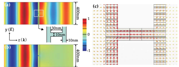
Fig. 2. (Color online) (a) The electromagnetic energy can be squeezed and tunneled through a two dimensional H-shape channel made from the ENZ meta-atom stacks, but (b) cannot be transmitted through a silica channel with the same geometry, where the magnetic field distribution is displayed at 455 THz. (c) The energy flow distribution near the central channel region illustrates the squeezing and tunneling phenomenon.
